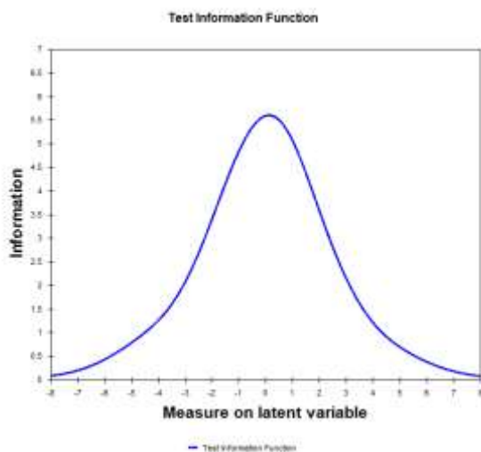
Test Information Function for The Two-Tier Multiple-Choice Test
